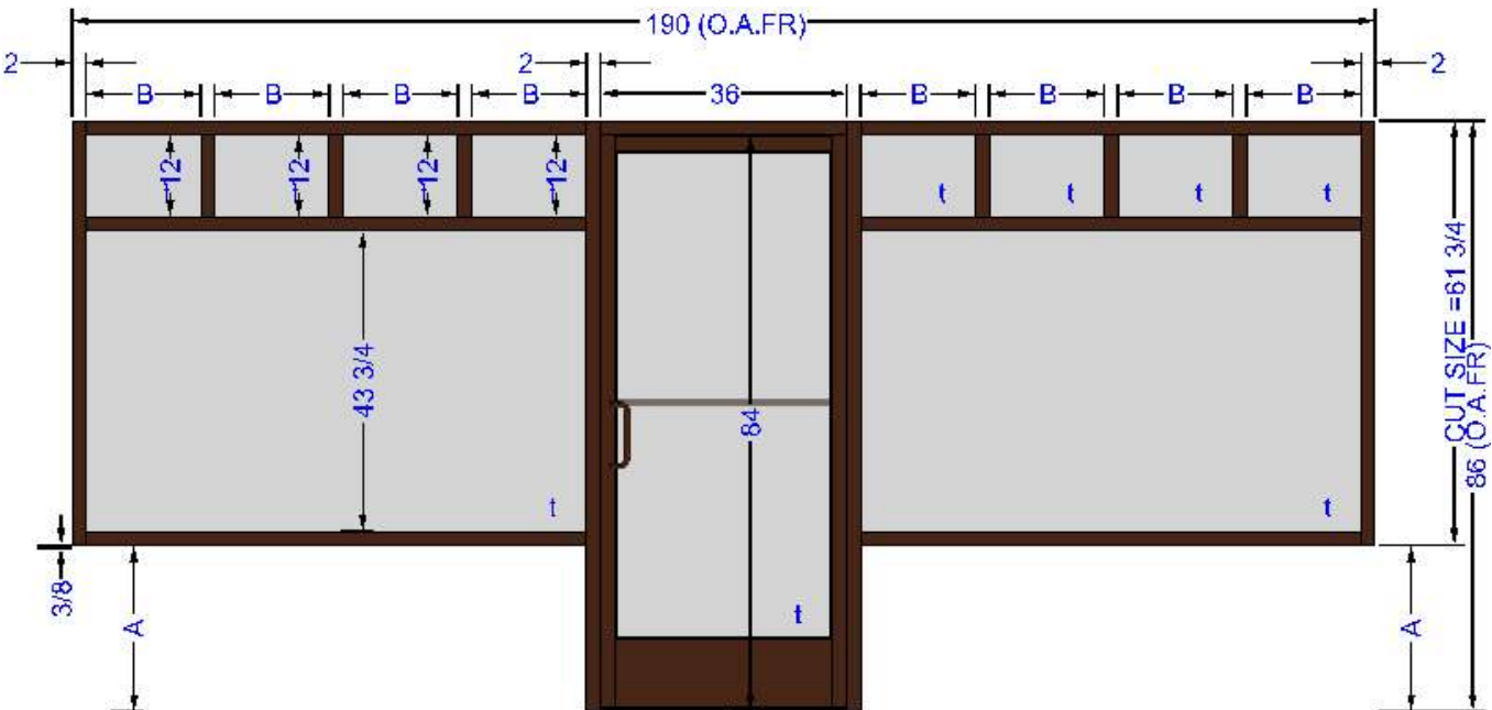
New Proposed Window Configuration, Now With Simulated Transoms
